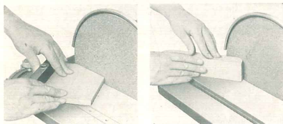
Plain and compound miters are easily sanded with the aid of the miter gage. Accurate work to layout lines accomplished with ease on this precision machine.
